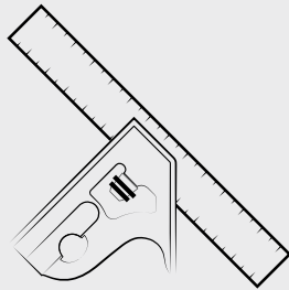
Combination Square
