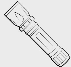
Flashlight
