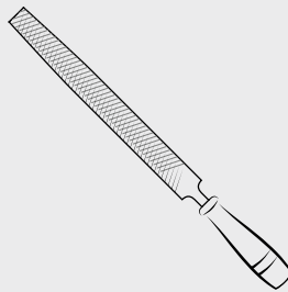
File
