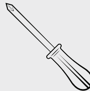
Screw Driver
